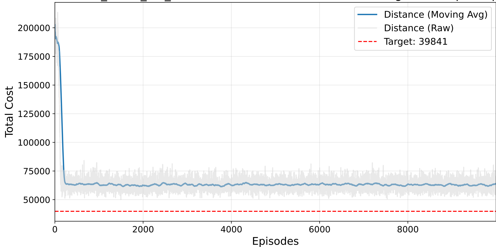
Final NO_MASK_NO_BAYESIAN Masked AutoRL-SOP Training - kro124p.2.sop
